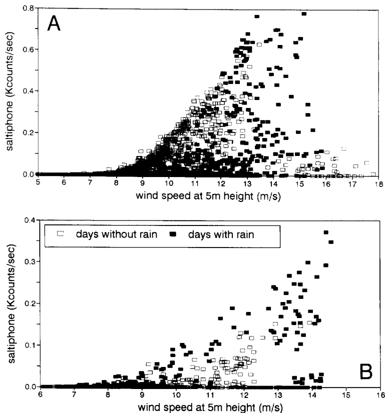
Fig. 4. Saltiphone counts (at 0.10 m height) versus wind speed (at 5 m height), for days with and without rainfall. (A) Schiermonnikoog (measuring period 3 March–27 May 1991); (B) Groote Keeten (measuring period 5–24 February 1992).
