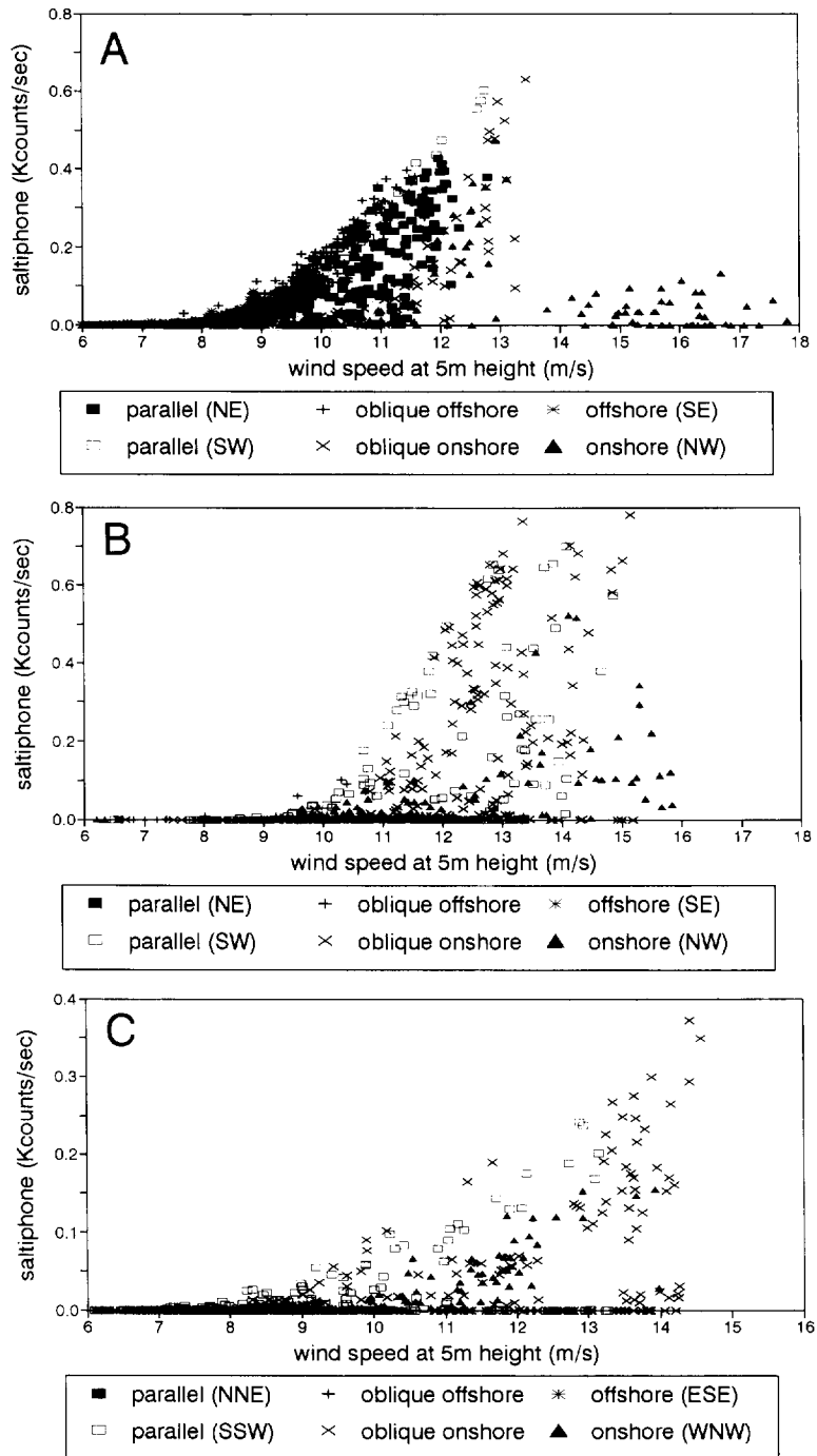
Fig. 6. Saltiphone counts versus wind speed, for several ranges of wind direction. (A) Schiermonnikoog, dry days; (B) Schiermonnikoog, wet days; (C) Grootte Keeten.
