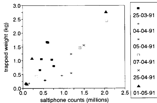
Fig. 3. Relationship between trapped weights (not corrected for trap-efficiency) and saltiphone counts over several periods. Amounts of sand trapped in period = 0.961 \times total number of Mcounts in period + 0.197; R^2 = 0.589 .
