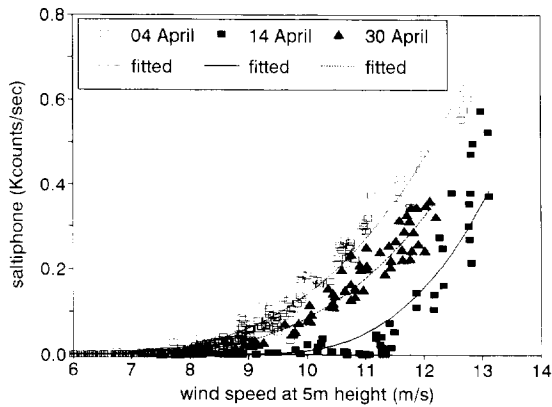
Fig. 5. Actual transport and fitted curves for potential transport (Eq. 1) for three days in April 1991, Schiermonnikoog. Predictions are based on curve-fitting procedure described below.
