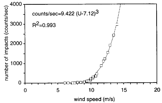
Fig. 2. Relationship between saltiphone counts and wind speed (after Van Dijk and Hollemans, 1991). Wind speed is measured at 0.35 m (centre of wind tunnel); impacts with the saltiphone were recorded at 0.03 m height.
