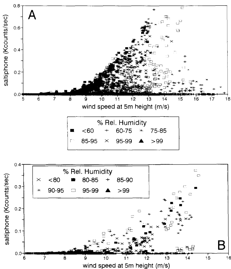
Fig. 7. Saltiphone counts versus wind speed, for several ranges of relative humidity. (A) Schiermonnikoog; (B) Groote Keeten.
