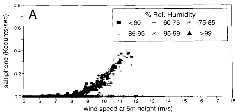
Fig. 8. Saltiphone counts versus wind speed, for several ranges of relative humidity: (A) offshore winds (60–210°); (B) parallel winds (210–240° and 30–60°), dry days; (C) id., wet days; (D) oblique onshore winds (240–285° and 345–30°), dry days; (E) id., wet days; (F) onshore winds (285–345°), dry days; (G) id., wet days.
