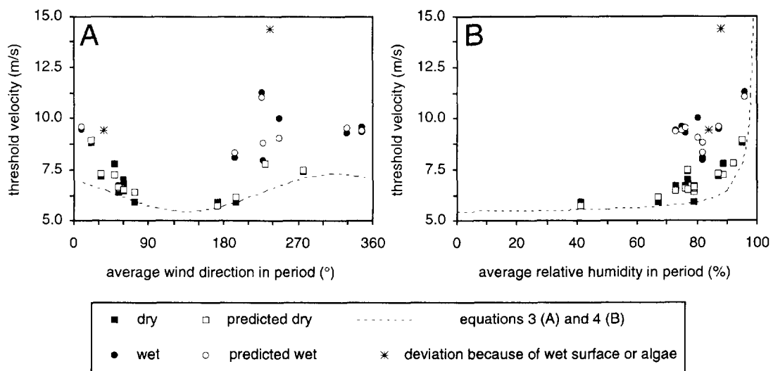
Fig. 9. Observed and predicted threshold velocities versus (A) wind direction and (B) relative humidity.
