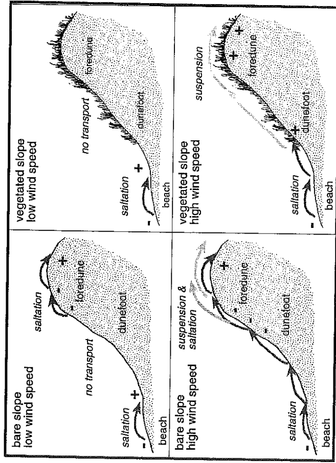
Figure 9.9. Conceptual scheme of landward transport over foredunes (from Arens 1996; with permission from Elsevier Science).
